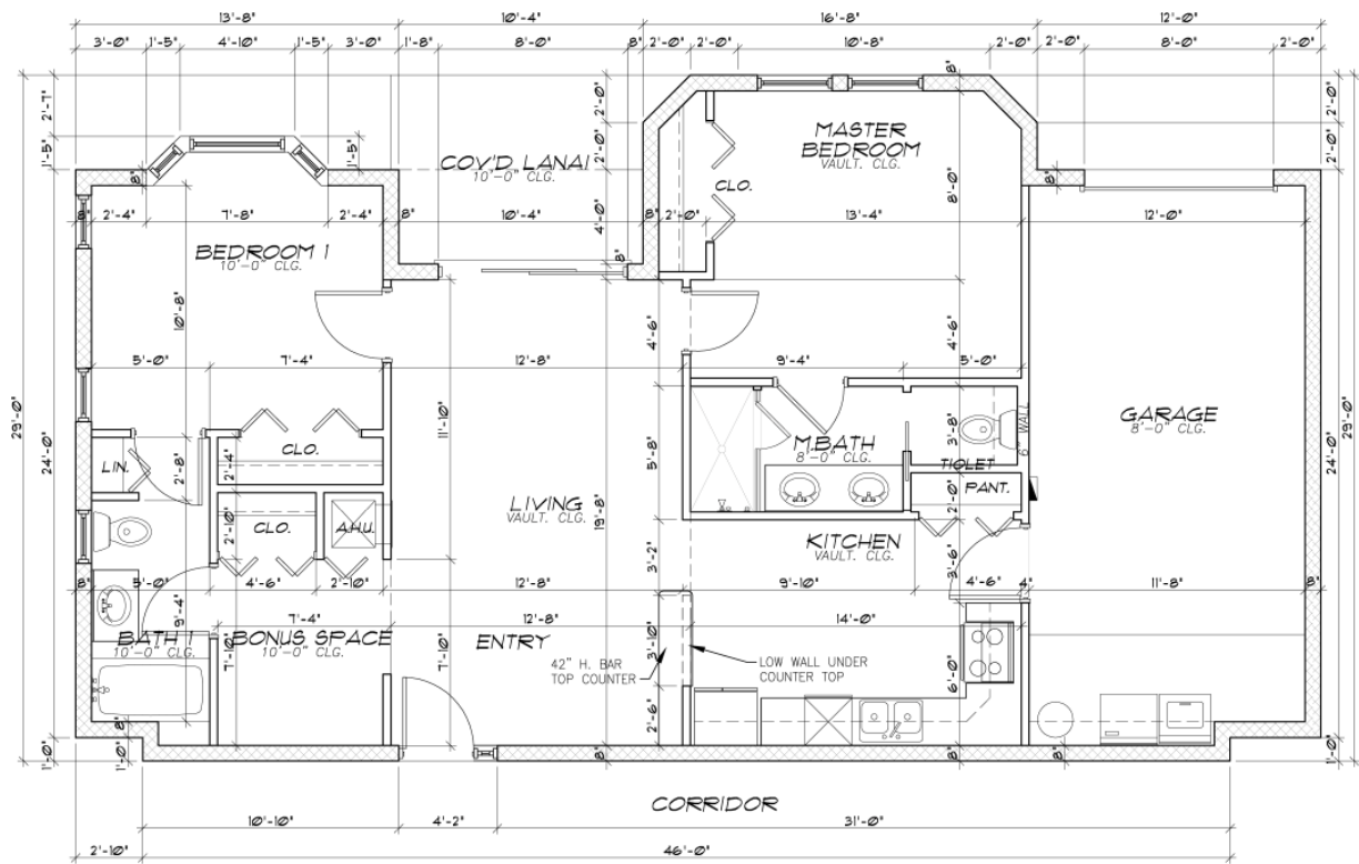
TYPICAL 2-BEDROOM FLOOR PLAN
